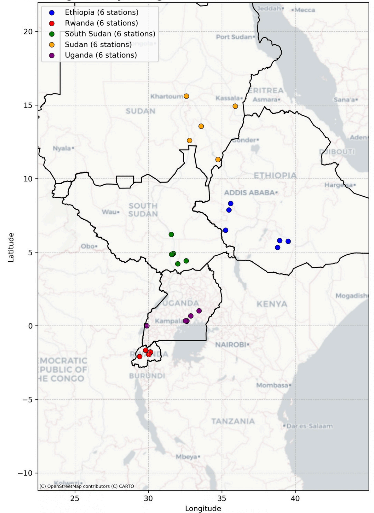
WHCA Regional Hydrological Station Network — Five Countries
